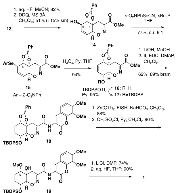
Scheme 4. Completion of the synthesis of trichodermamide B. DDQ=2,3-Dicyano-5,6-dichloro-parabenzquinone, sm=starting material, EDC=1-ethyl-3-(3-dimethylaminopropyl)carbodiimide hydrochloride, DMAP=4-dimethylaminopyridine, Py=pyridine, brsm=based on recovered starting material, TBDSPOTf= tert -butyldi-phenylsilyl trifluoromethanesulfonate.
